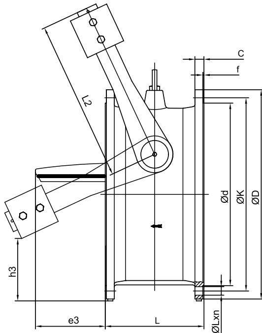
FIG. 5 Tilting Disc Check Valve Side View
