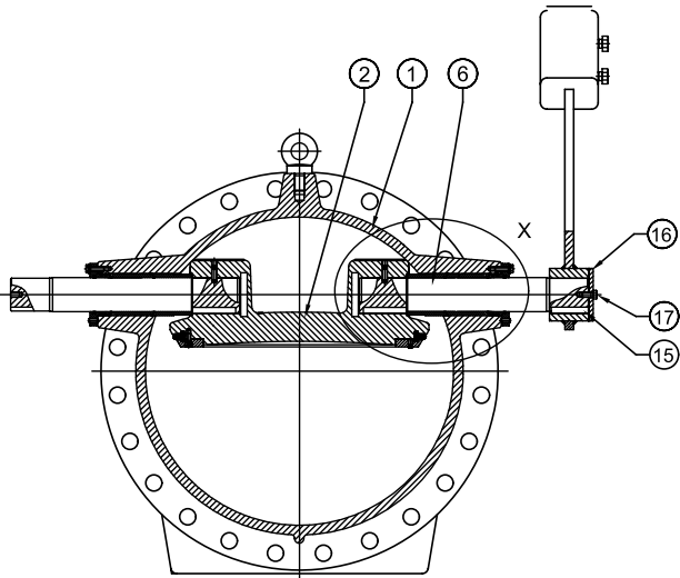
FIG. 2 Opened Position
